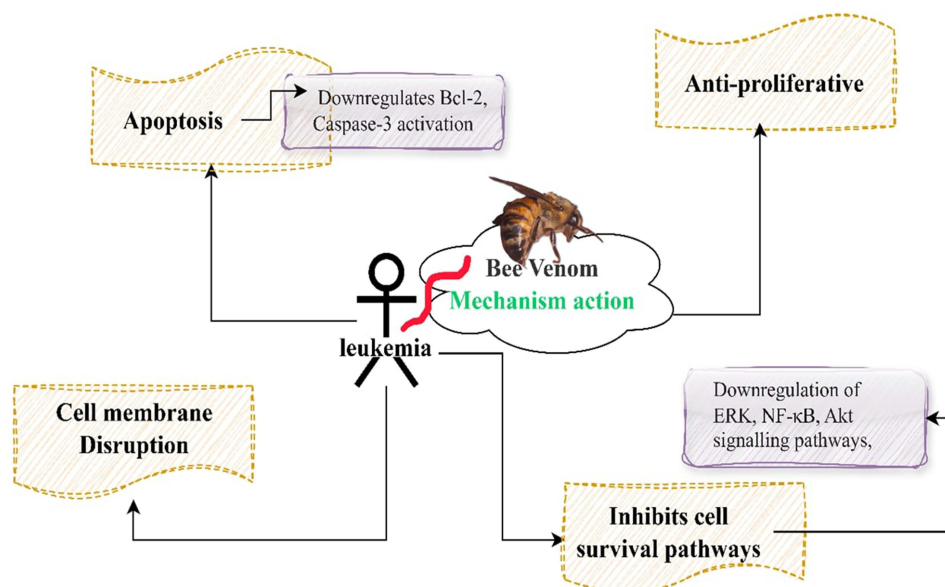
Figure 3 Mechanism action of BV against leukemia (Created with draw.io).
